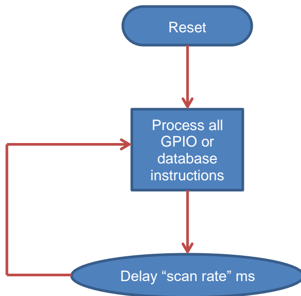
Figure 2: GPIO / Database Logic Scan Cycle
