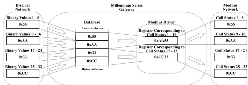
Figure 15: BACnet - Modbus (Binary Objects & Discretes) Little Endian
